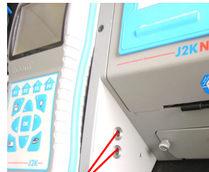
Connections for pitot tube
